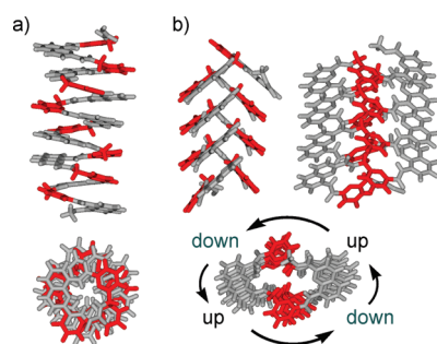
FIGURE 1. Side view and top view of energy minimized conformations (MacroModel v8.6; force field MM3) of (PQ) 8 as a canonical helix (a) and as a noncanonical "herringbone" helix (b). Amide and quinoline moieties are shown in gray; 6-aminomethyl-pyridine units are shown in red.
